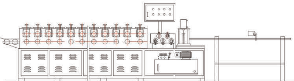
Roll Forming Main Machine
